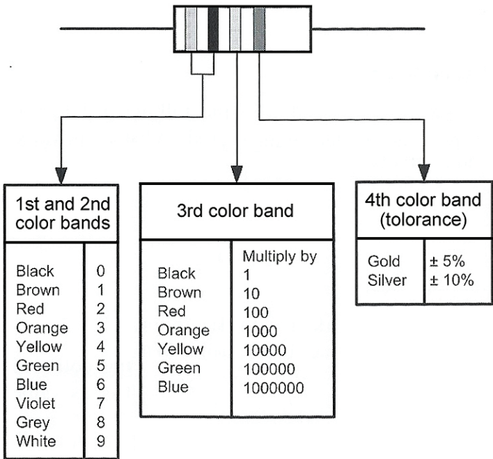
Four band resistor color code
